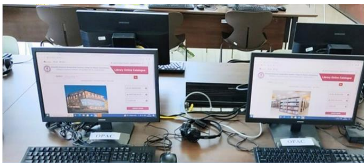
OPAC Search
